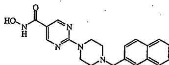
.083 CF 3 COOH compound 6
